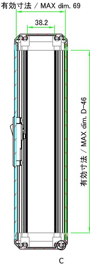
B-B (1:3)
